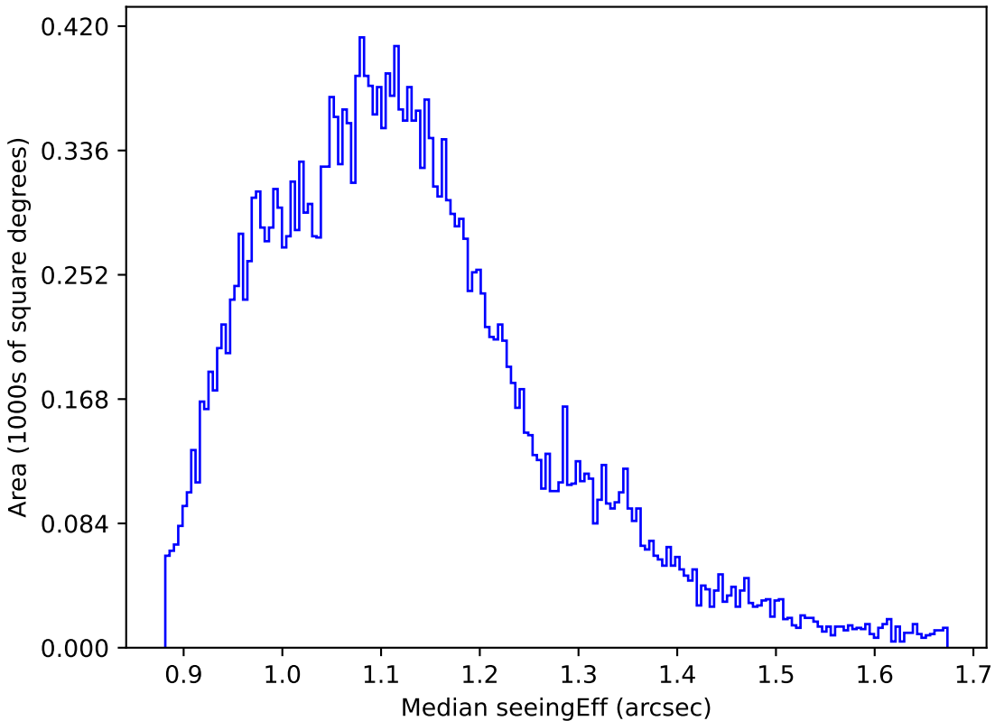
ddf_loaded_half_fl1_v3.4_10yrs All sky g band: Median seeingEff
