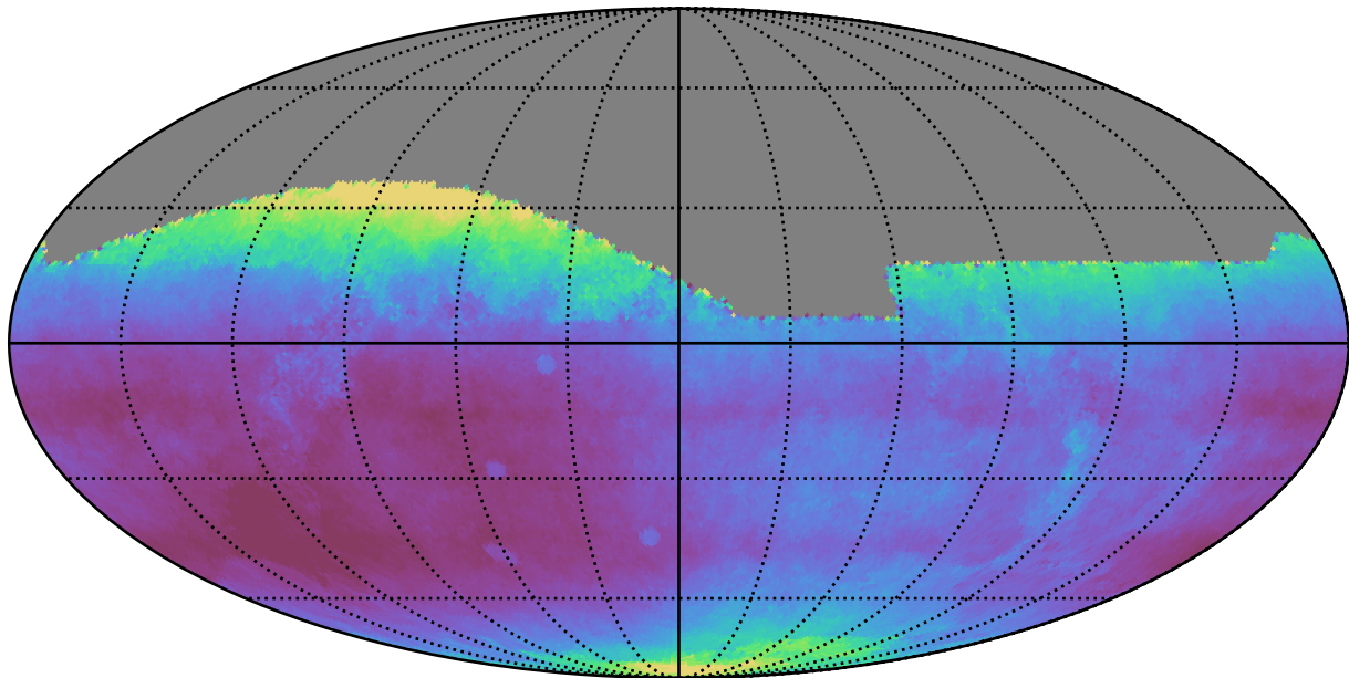
ddf_loaded_half_fl1_v3.4_10yrs All sky all bands: Median seeingEff
