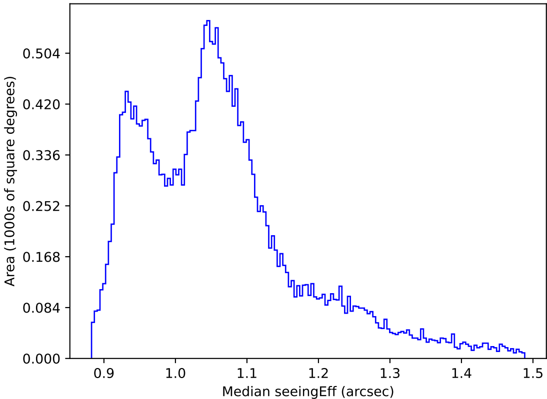
ddf_loaded_half_fl1_v3.4_10yrs All sky all bands: Median seeingEff
