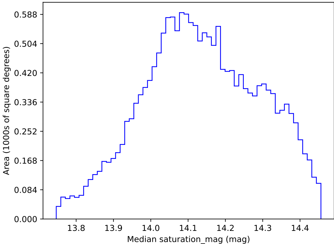
ddf_loaded_half_fl1_v3.4_10yrs WFD z band: Median saturation_mag
