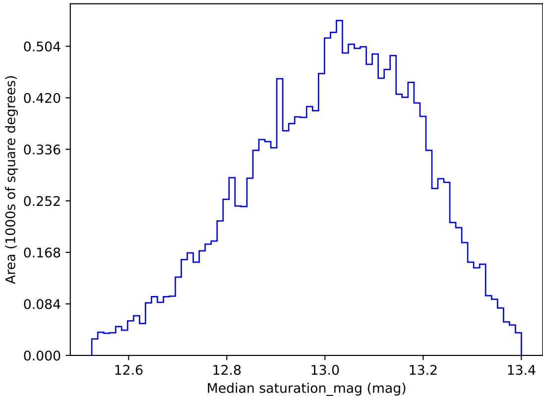
ddf_loaded_half_fl1_v3.4_10yrs WFD u band: Median saturation_mag
