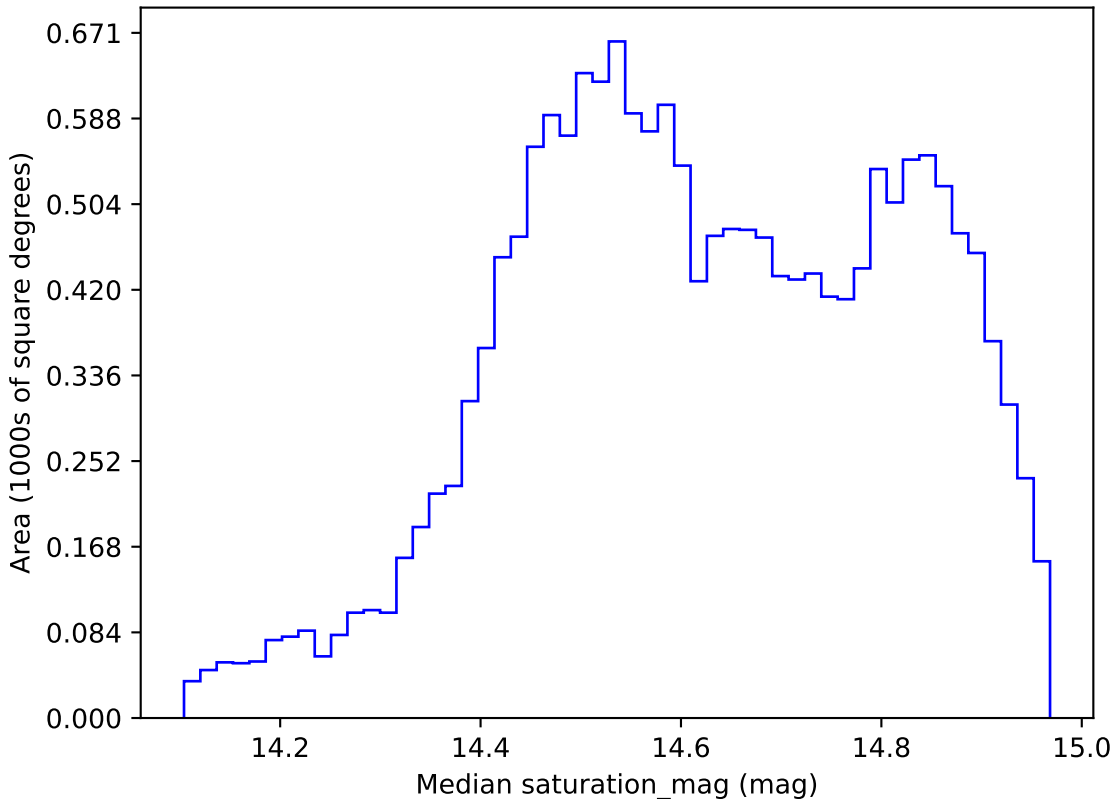
ddf_loaded_half_fl1_v3.4_10yrs WFD r band: Median saturation_mag
