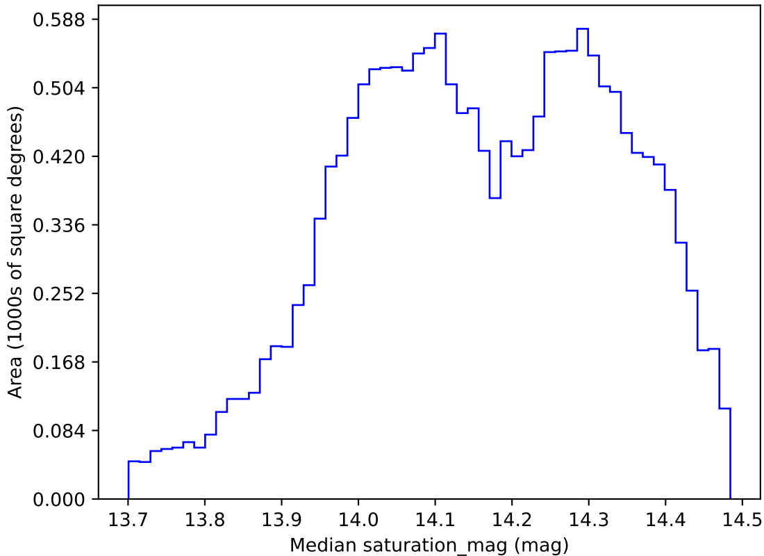
ddf_loaded_half_fl1_v3.4_10yrs WFD all bands: Median saturation_mag
