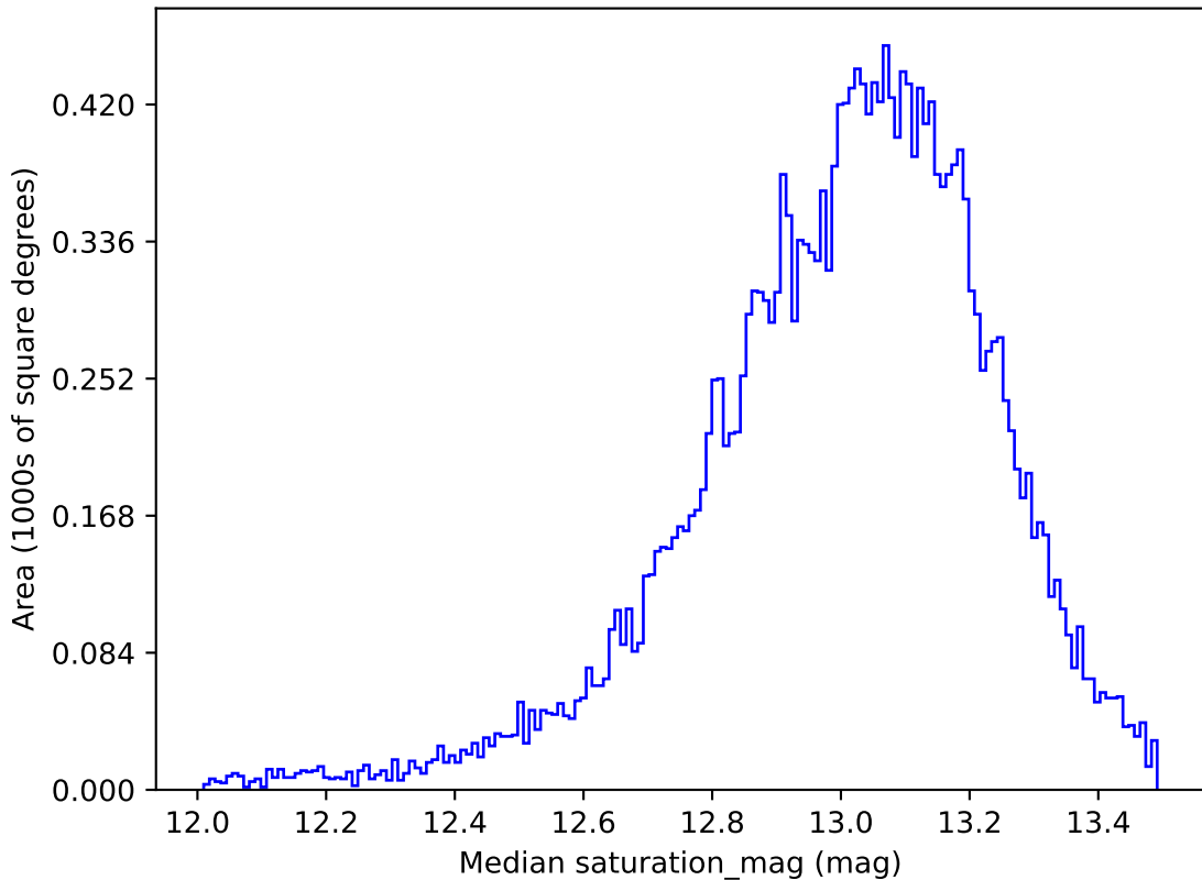
ddf_loaded_half_fl1_v3.4_10yrs All sky u band: Median saturation_mag
