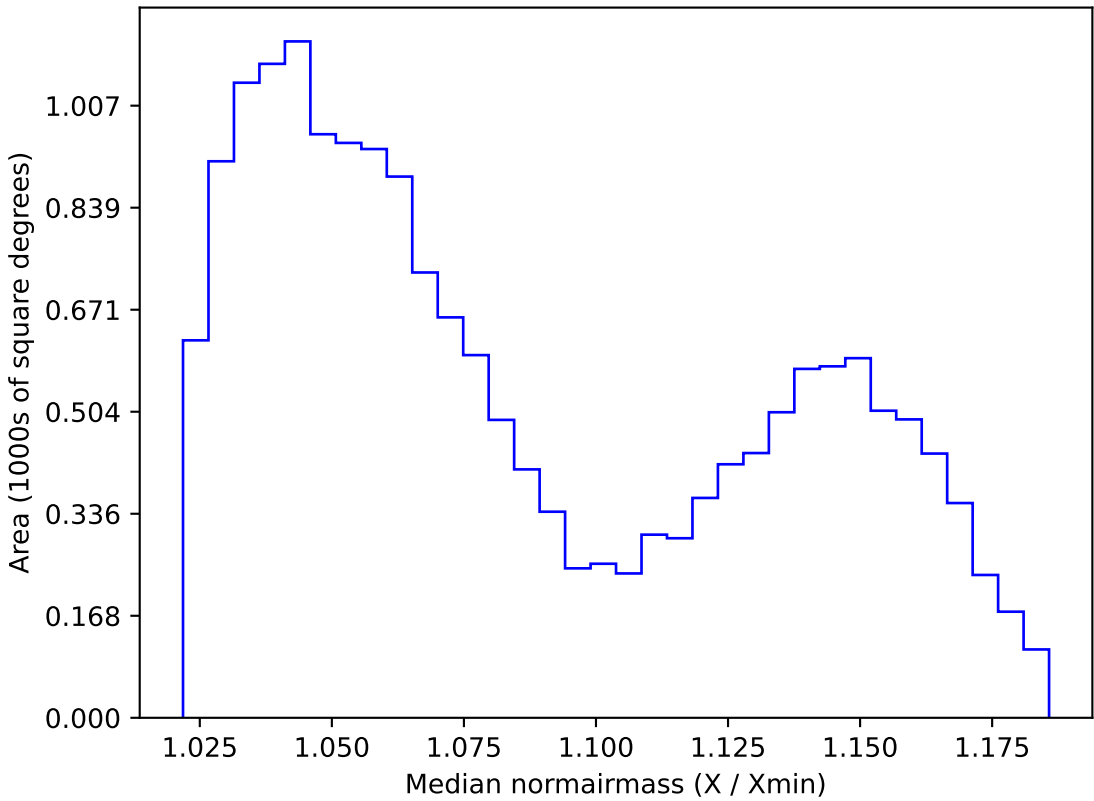
ddf_loaded_half_fl1_v3.4_10yrs WFD z band: Median normairmass
