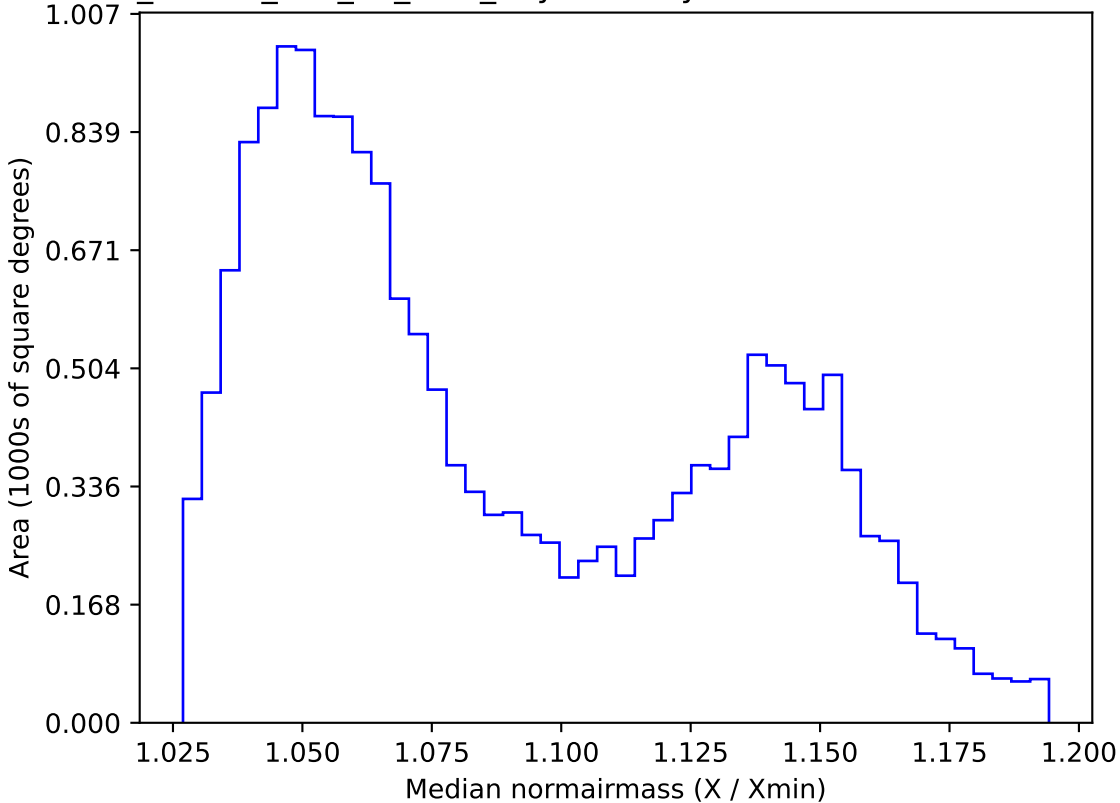
ddf_loaded_half_fl1_v3.4_10yrs WFD y band: Median normairmass
