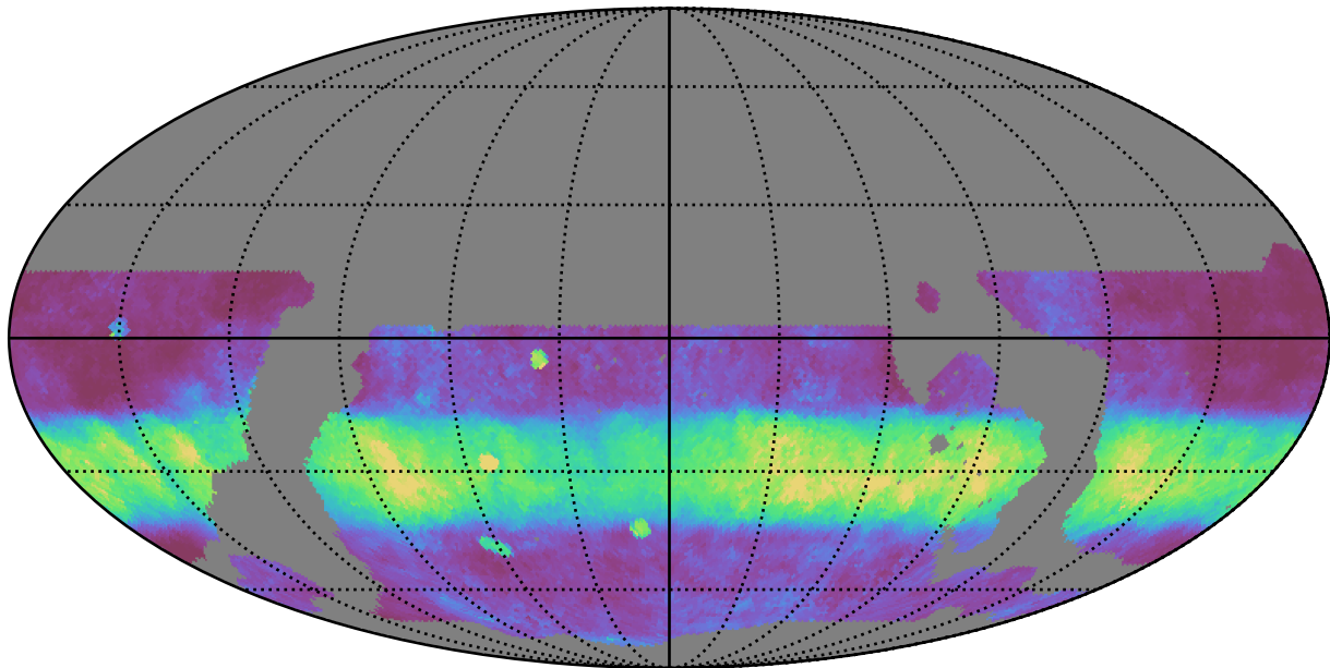
ddf_loaded_half_fl1_v3.4_10yrs WFD r band: Median normairmass
