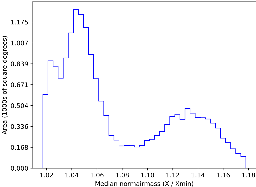
ddf_loaded_half_fl1_v3.4_10yrs WFD r band: Median normairmass
