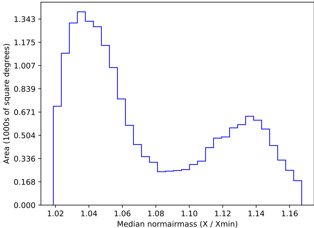
ddf_loaded_half_fl1_v3.4_10yrs WFD i band: Median normairmass
