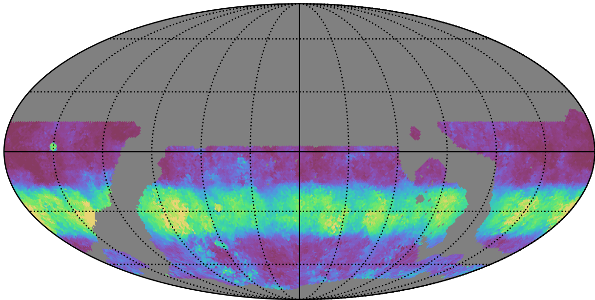
ddf_loaded_half_fl1_v3.4_10yrs WFD g band: Median normairmass
