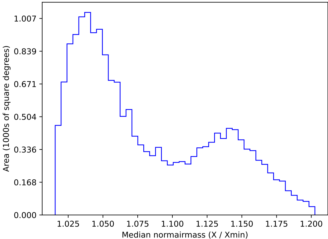
ddf_loaded_half_fl1_v3.4_10yrs WFD g band: Median normairmass
