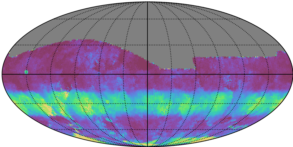
ddf_loaded_half_fl1_v3.4_10yrs All sky g band: Median normairmass
