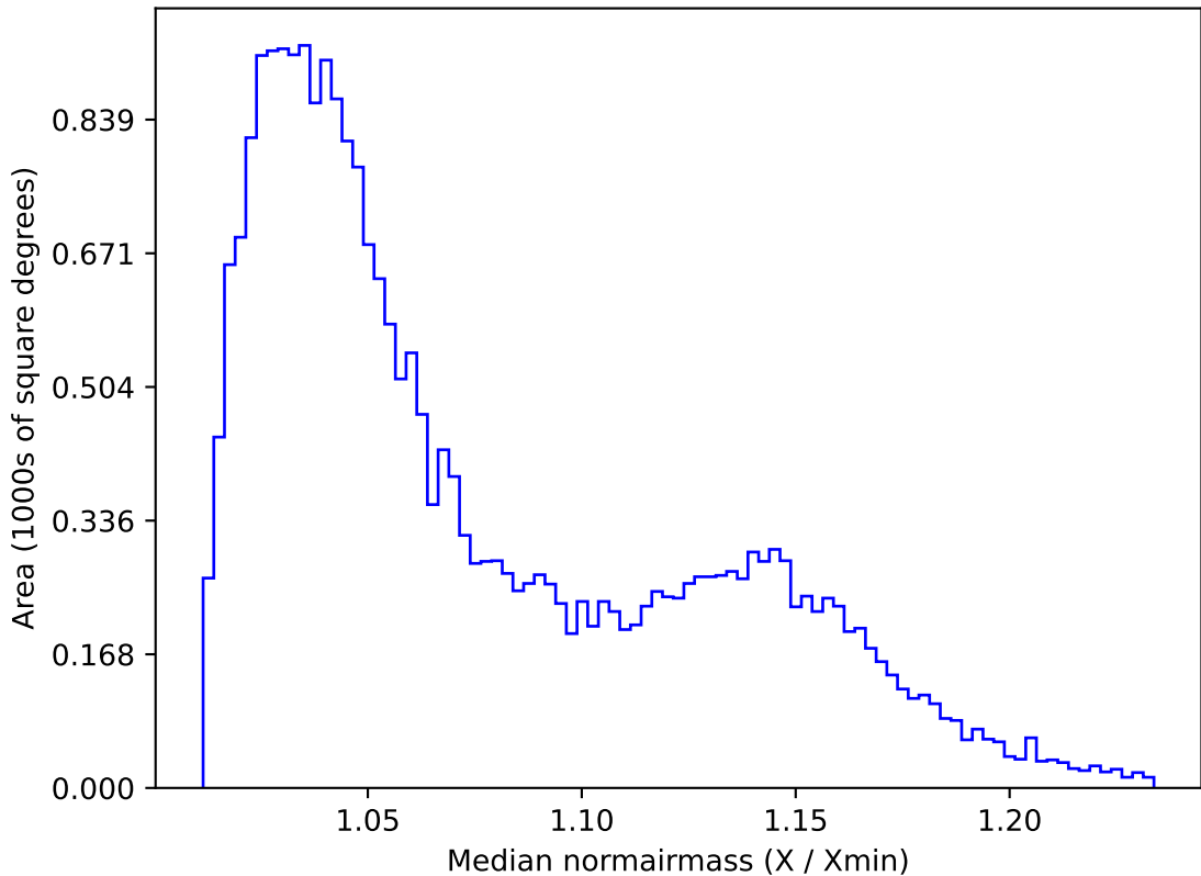
ddf_loaded_half_fl1_v3.4_10yrs All sky g band: Median normairmass
