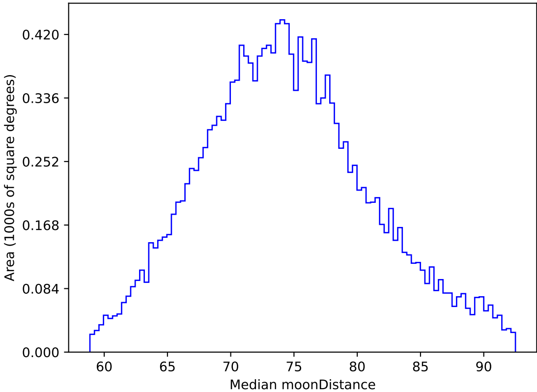
ddf_loaded_half_fl1_v3.4_10yrs WFD z band: Median moonDistance
