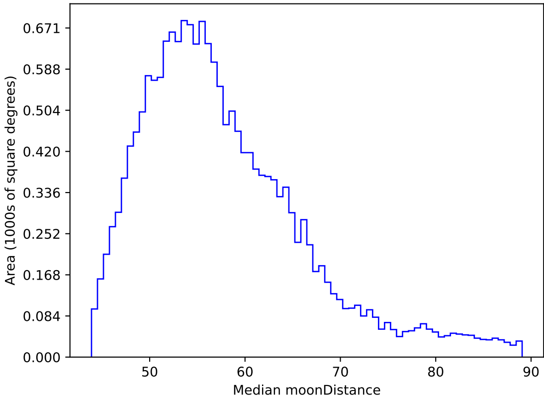
ddf_loaded_half_fl1_v3.4_10yrs WFD y band: Median moonDistance
