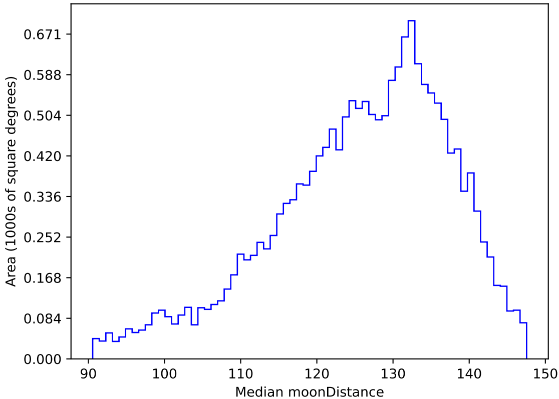
ddf_loaded_half_fl1_v3.4_10yrs WFD u band: Median moonDistance
