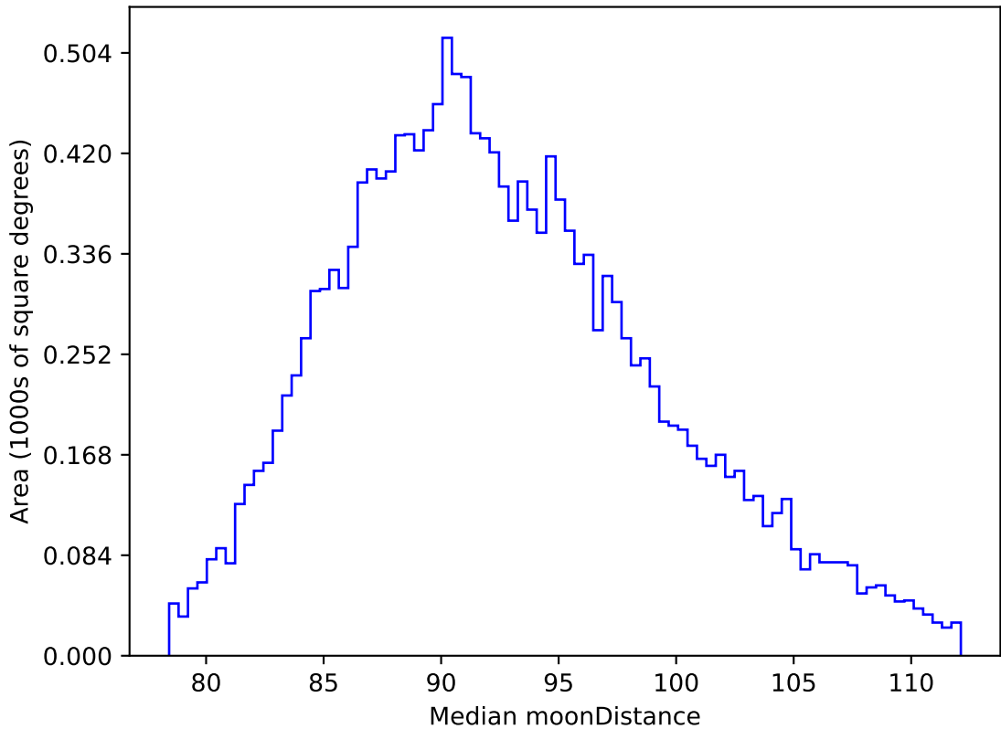
ddf_loaded_half_fl1_v3.4_10yrs WFD i band: Median moonDistance
