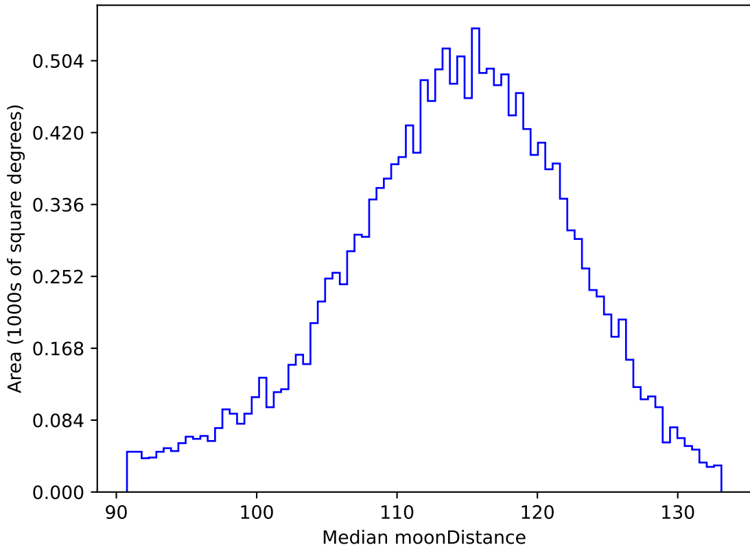
ddf_loaded_half_fl1_v3.4_10yrs WFD g band: Median moonDistance
