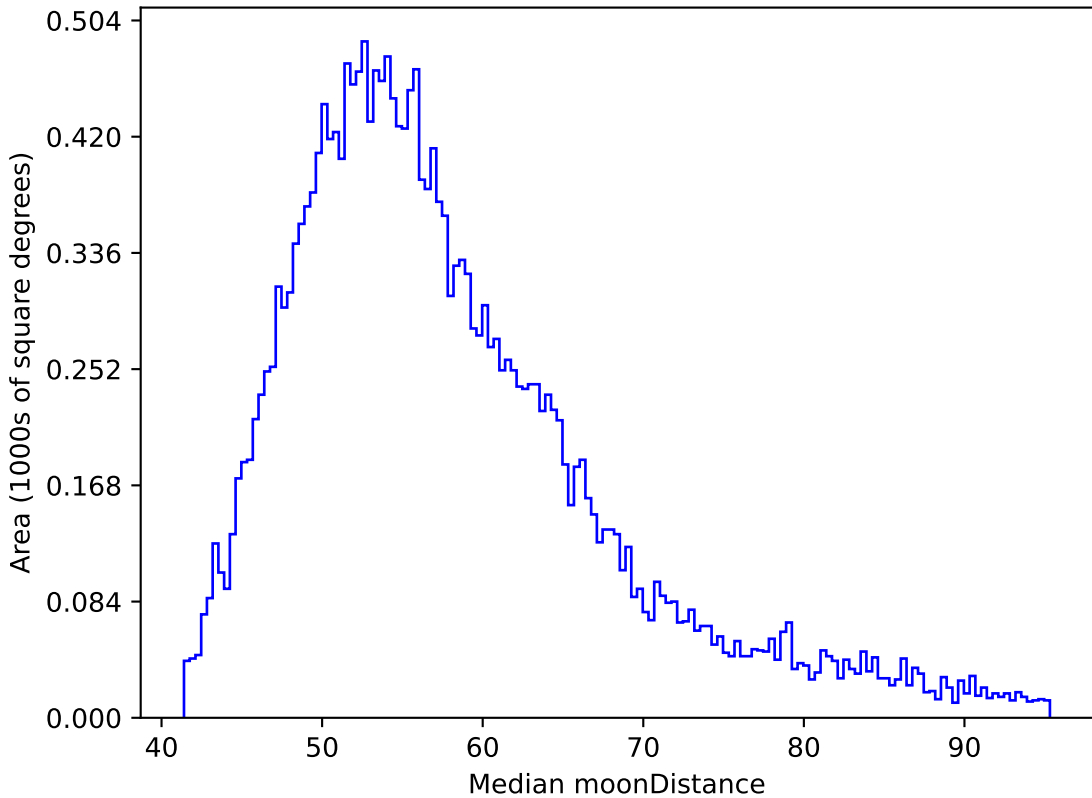
ddf_loaded_half_fl1_v3.4_10yrs All sky y band: Median moonDistance
