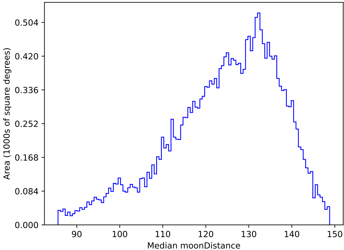
ddf_loaded_half_fl1_v3.4_10yrs All sky u band: Median moonDistance
