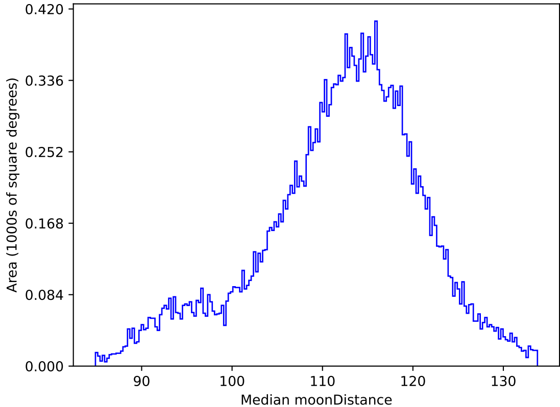
ddf_loaded_half_fl1_v3.4_10yrs All sky r band: Median moonDistance
