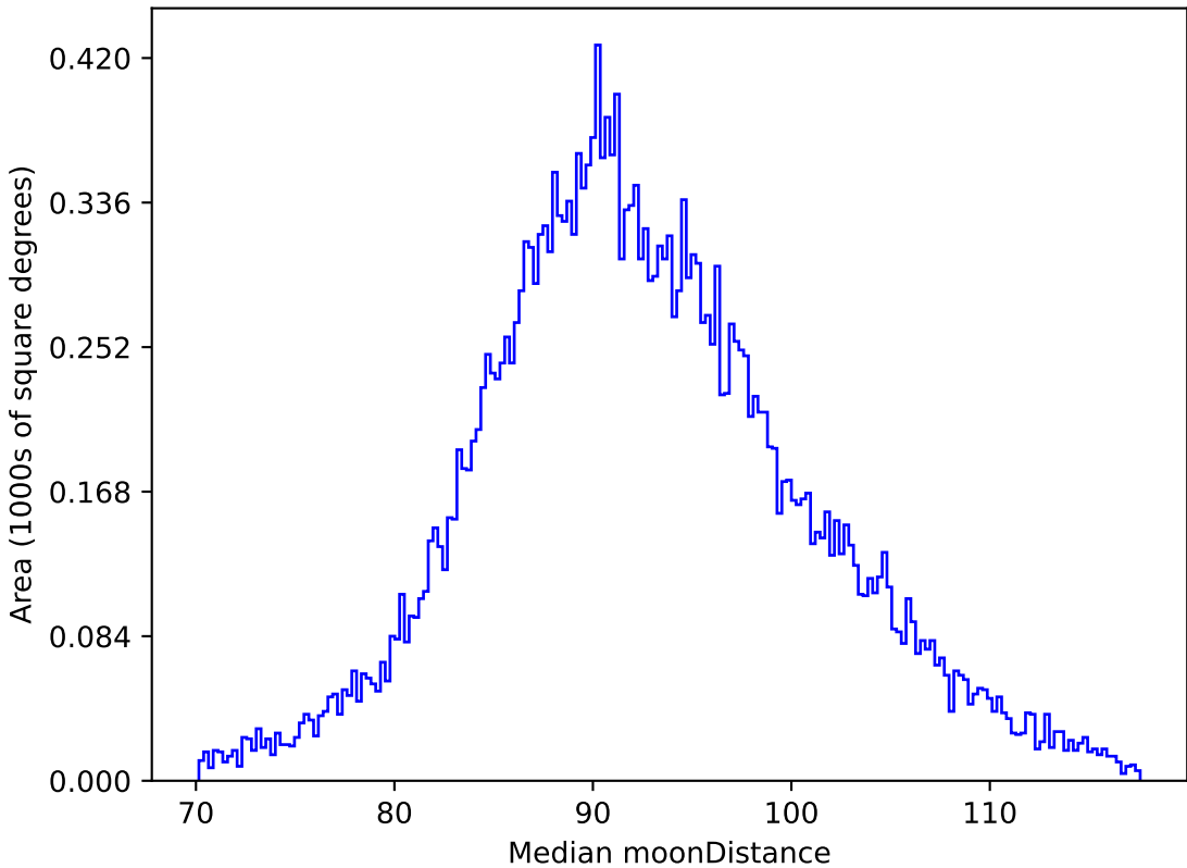
ddf_loaded_half_fl1_v3.4_10yrs All sky i band: Median moonDistance
