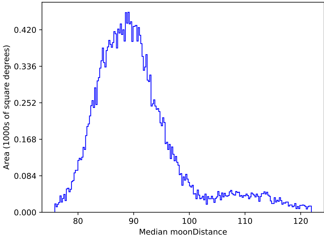
ddf_loaded_half_fl1_v3.4_10yrs All sky all bands: Median moonDistance
