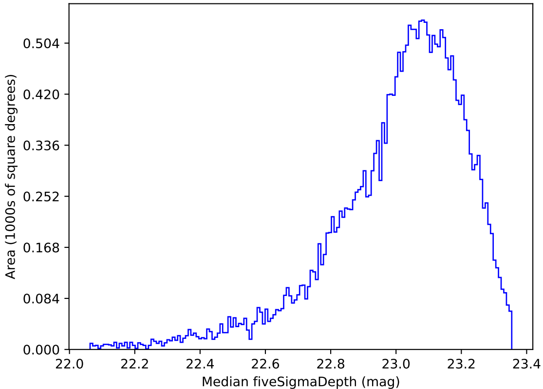
ddf_loaded_half_fl1_v3.4_10yrs Yr 1 z band: Median fiveSigmaDepth
