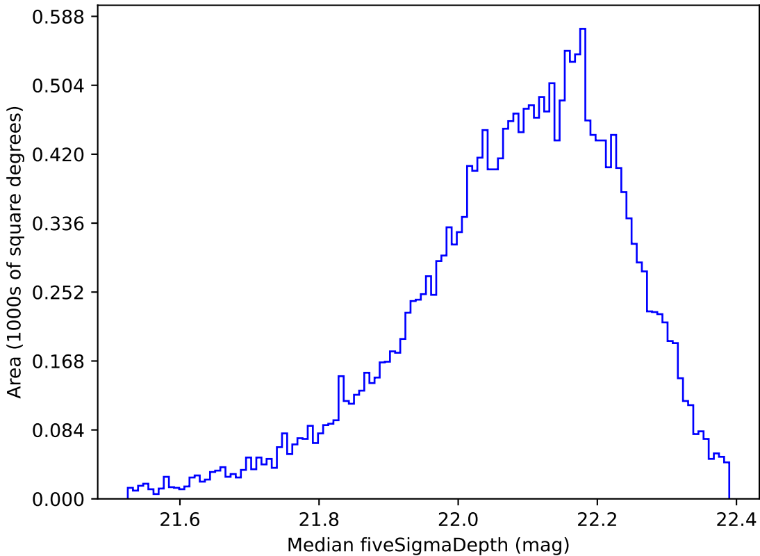
ddf_loaded_half_fl1_v3.4_10yrs Yr 1 y band: Median fiveSigmaDepth
