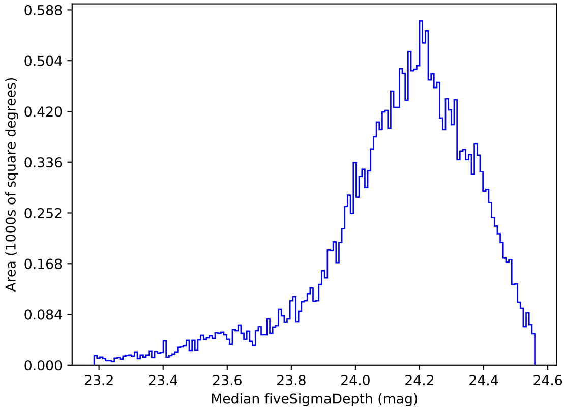
ddf_loaded_half_fl1_v3.4_10yrs Yr 1 r band: Median fiveSigmaDepth
