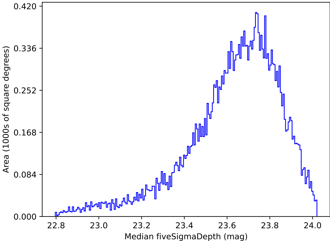
ddf_loaded_half_fl1_v3.4_10yrs Yr 1 i band: Median fiveSigmaDepth
