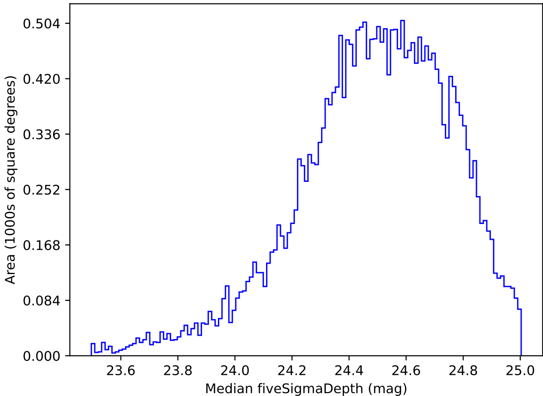
ddf_loaded_half_fl1_v3.4_10yrs Yr 1 g band: Median fiveSigmaDepth
