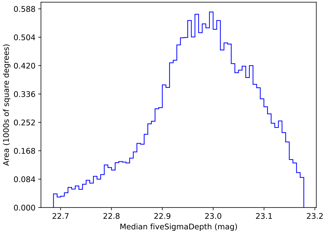
ddf_loaded_half_fl1_v3.4_10yrs WFD z band: Median fiveSigmaDepth
