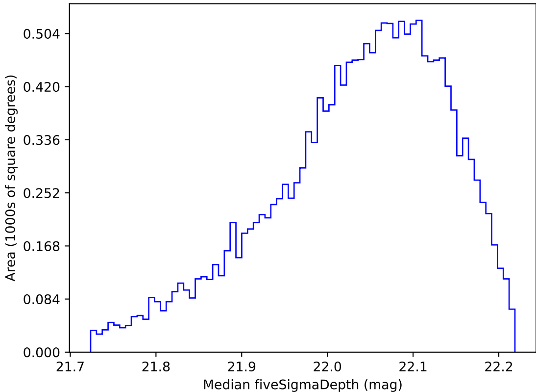
ddf_loaded_half_fl1_v3.4_10yrs WFD y band: Median fiveSigmaDepth
