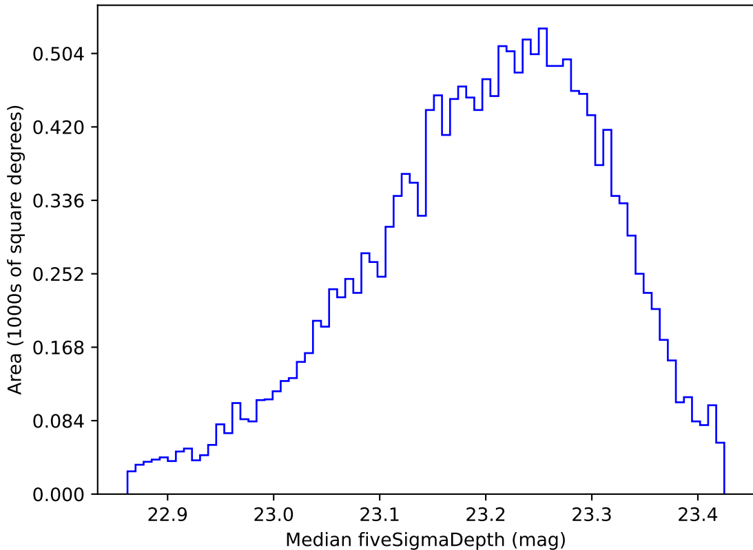
ddf_loaded_half_fl1_v3.4_10yrs WFD u band: Median fiveSigmaDepth
