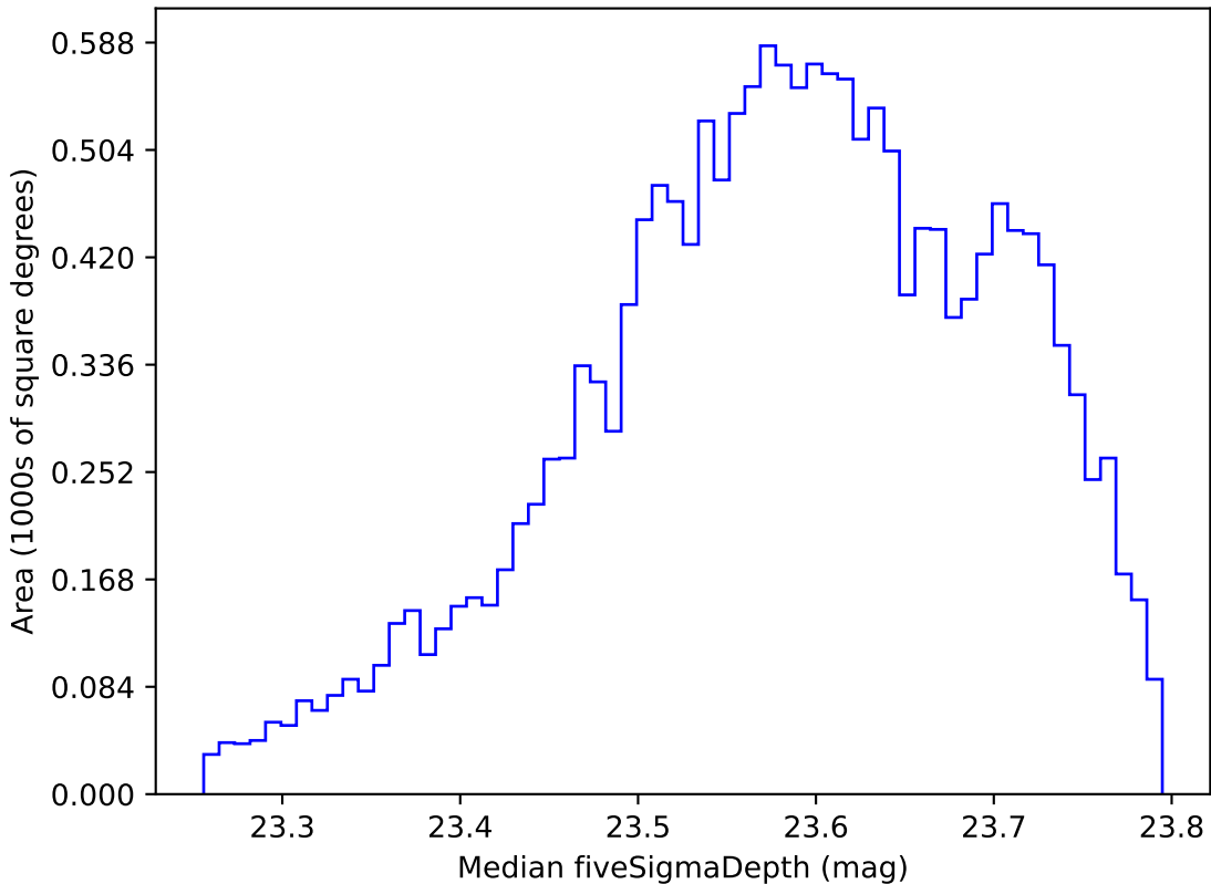
ddf_loaded_half_fl1_v3.4_10yrs WFD i band: Median fiveSigmaDepth
