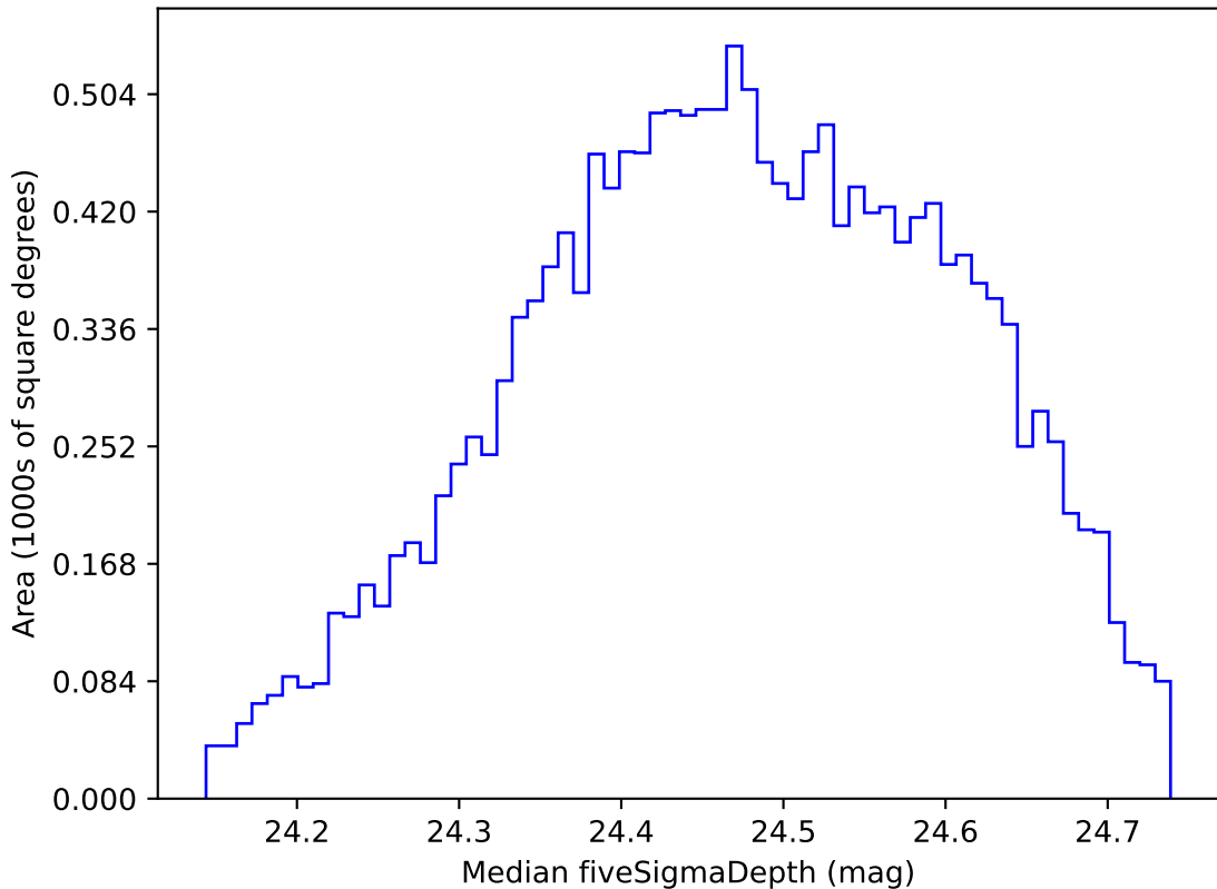
ddf_loaded_half_fl1_v3.4_10yrs WFD g band: Median fiveSigmaDepth
