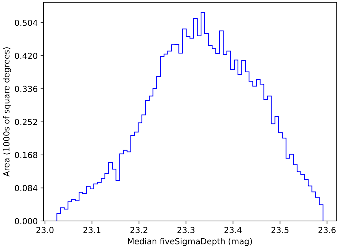
ddf_loaded_half_fl1_v3.4_10yrs WFD all bands: Median fiveSigmaDepth
