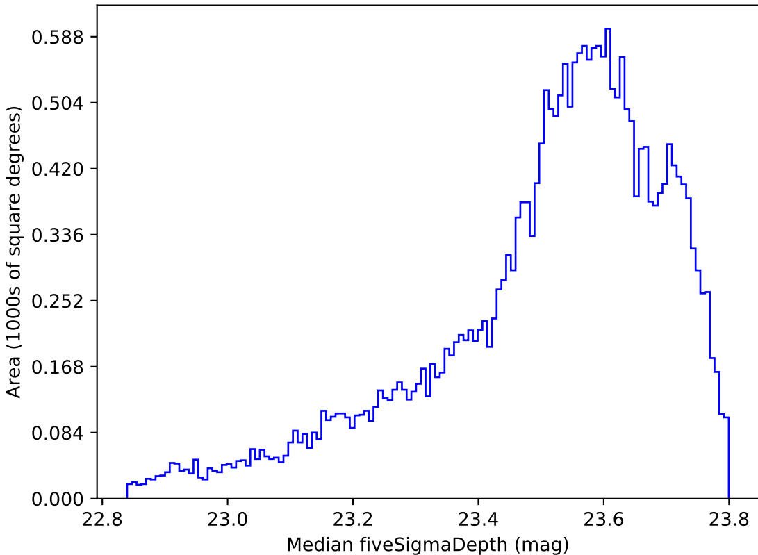
ddf_loaded_half_fl1_v3.4_10yrs All sky i band: Median fiveSigmaDepth
