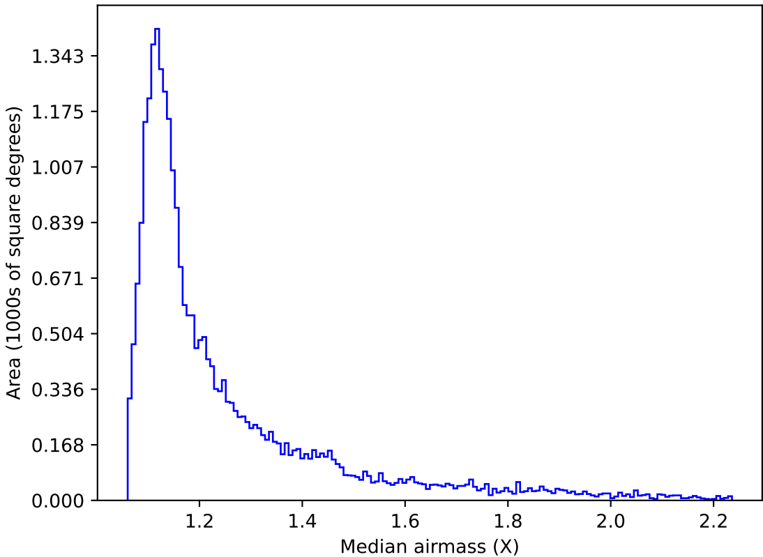
ddf_loaded_half_fl1_v3.4_10yrs Yr 1 z band: Median airmass
