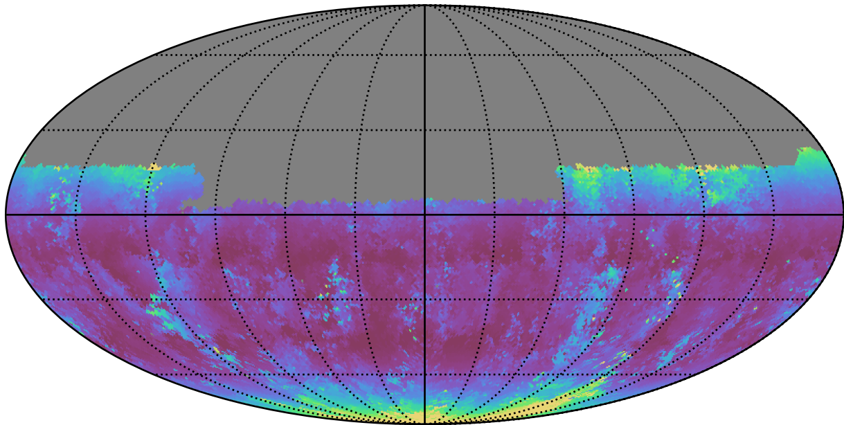
ddf_loaded_half_fl1_v3.4_10yrs Yr 1 u band: Median airmass
