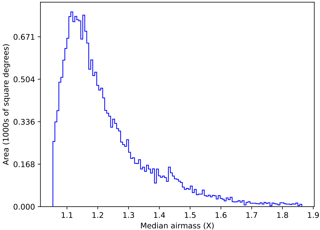
ddf_loaded_half_fl1_v3.4_10yrs Yr 1 u band: Median airmass
