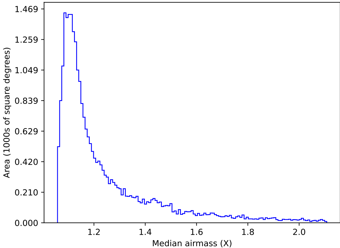
ddf_loaded_half_fl1_v3.4_10yrs Yr 1 r band: Median airmass
