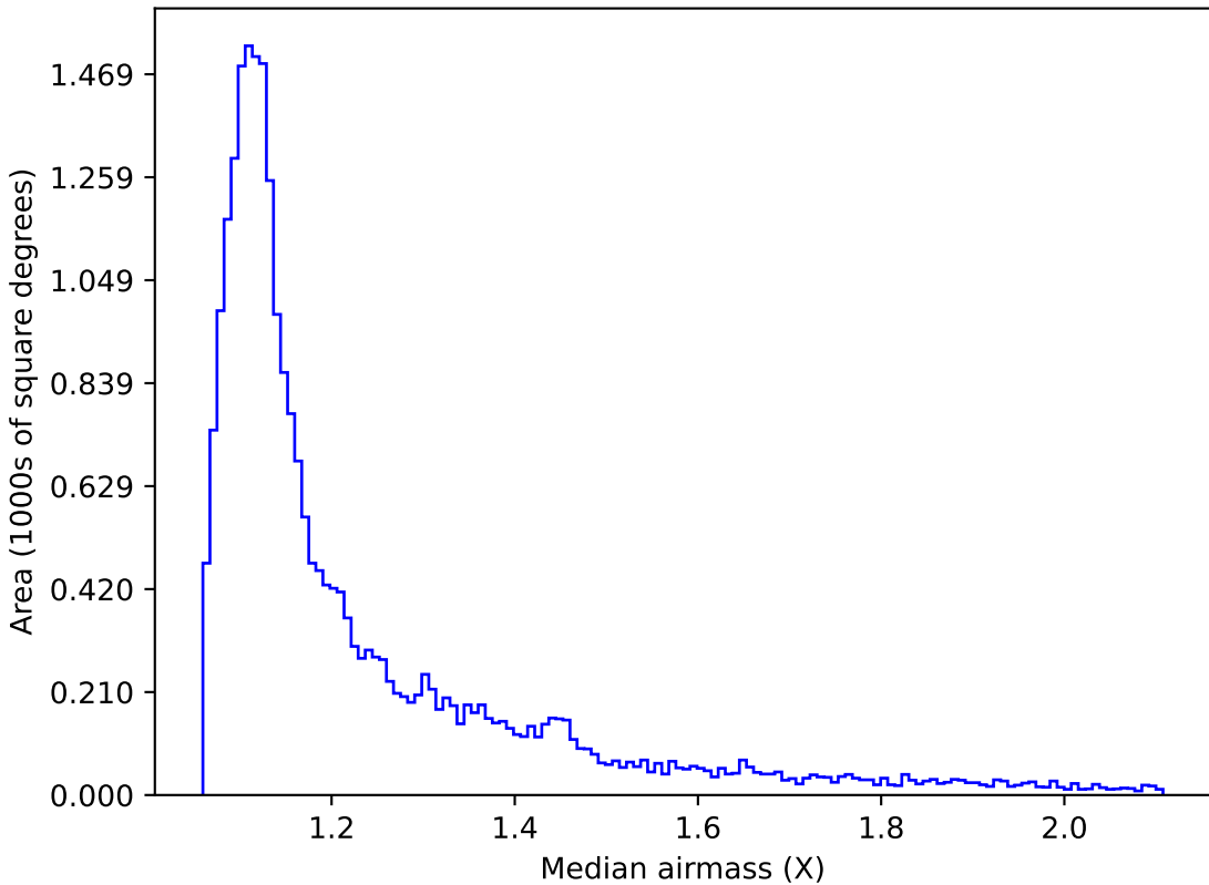
ddf_loaded_half_fl1_v3.4_10yrs Yr 1 i band: Median airmass
