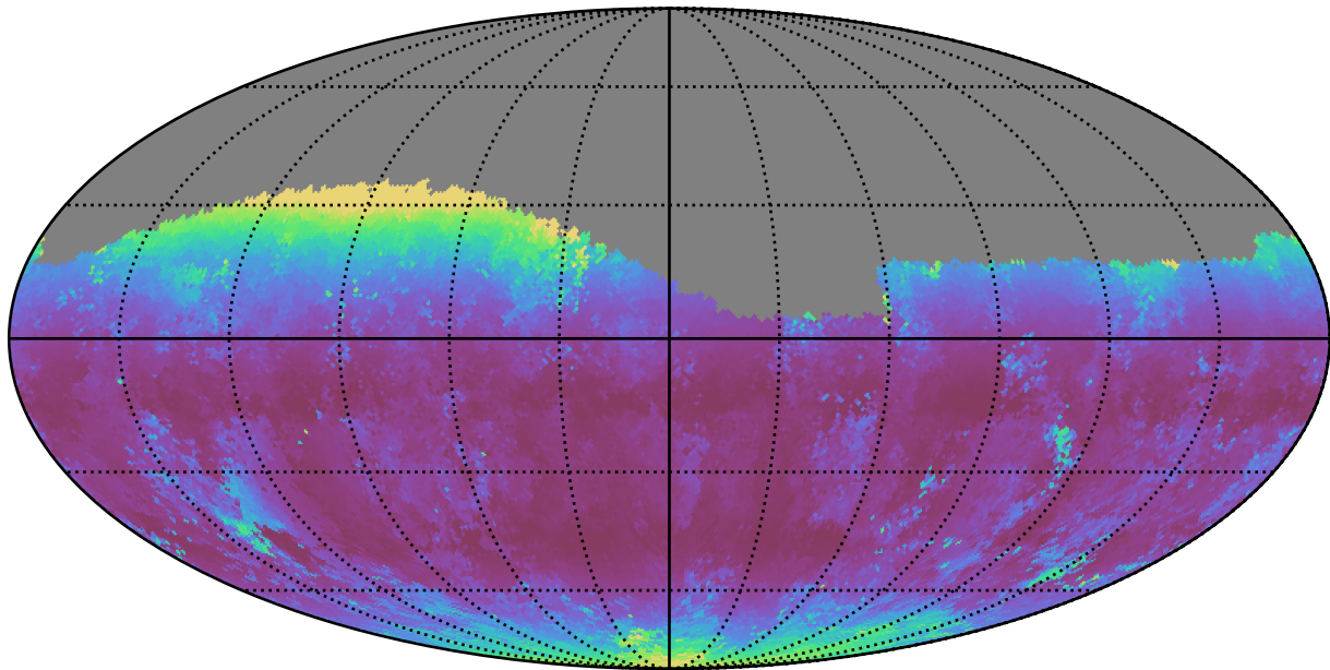
ddf_loaded_half_fl1_v3.4_10yrs Yr 1 g band: Median airmass
