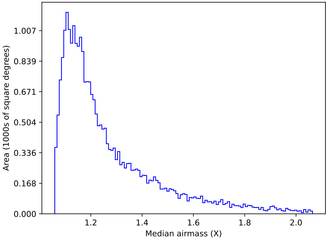
ddf_loaded_half_fl1_v3.4_10yrs Yr 1 g band: Median airmass
