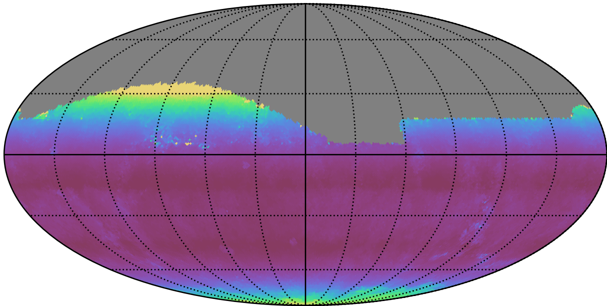
ddf_loaded_half_fl1_v3.4_10yrs Yr 1 all bands: Median airmass
