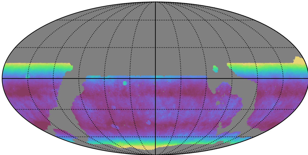
ddf_loaded_half_fl1_v3.4_10yrs WFD z band: Median airmass
