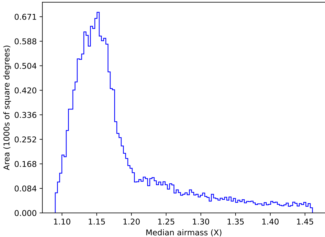
ddf_loaded_half_fl1_v3.4_10yrs WFD z band: Median airmass
