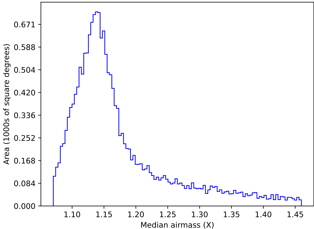
ddf_loaded_half_fl1_v3.4_10yrs WFD u band: Median airmass
